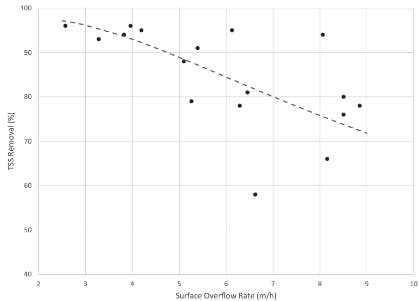
Figure 4.44 Effect of SOR on TSS removals during CEPT (Melcer, 2005, 2014; Fitzpatrick, 2012).
