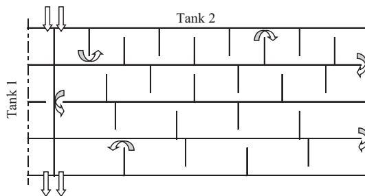
Figure 7.6 Horizontal baffled flocculation tanks.
