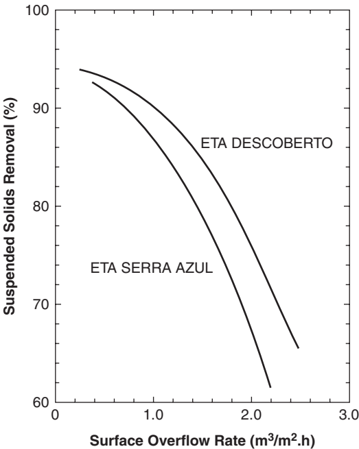
Figure B.7 Settling characteristics of filter backwash solids (Bratby, 1988).
