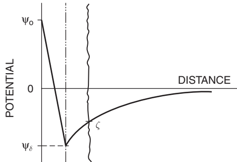
Figure 2.6 With polyvalent or surface-active counter-ions, reversal of charge may take place within the Stern layer.
