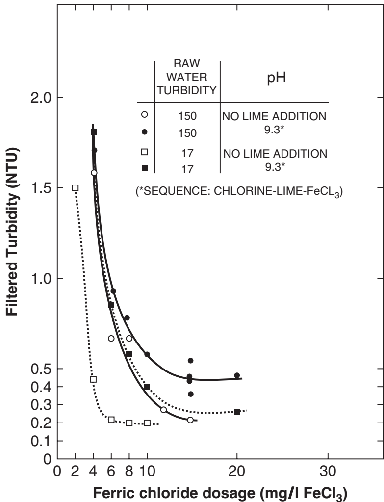
Figure 4.50 Filtered water qualities at low and high pH (Bratby, 1990).
