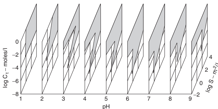
Figure 4.4 Zones of destabilization and restabilization as related to pH, colloid concentration, S and coagulant dosage, C_t . (From Stumm & O'Melia, 1968).
