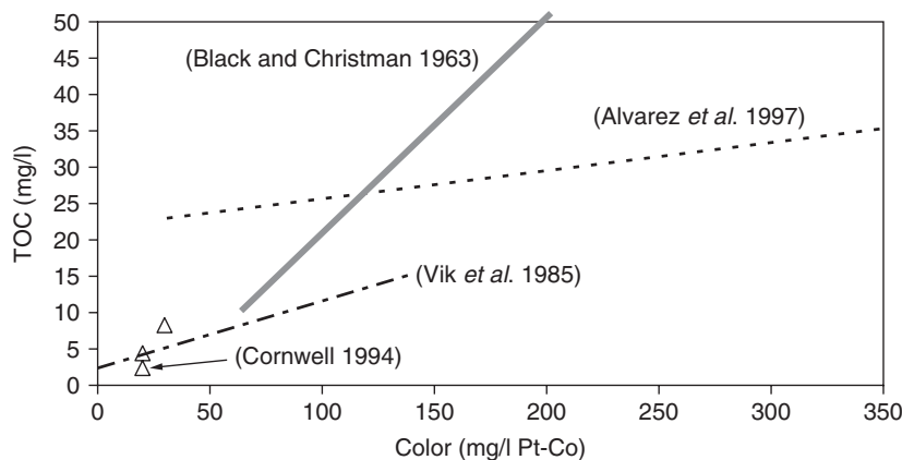
Figure 4.19 Examples of relationships between color and TOC (data derived from references shown).
