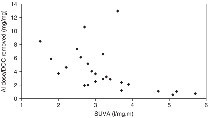
Figure 4.15 Influence of SUVA on alum (as Al) requirements for DOC removal.
