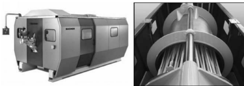
Figure B.26 Dehydri TM twist press (Courtesy Infilco Degremont Inc.: www.degremont-technologies.com ).
