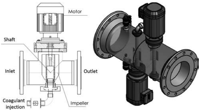
Figure 6.12 Example of in-line mixer with varying velocity gradient (courtesy Aquen Aqua-Engineering GmbH, www.aquen.de ).
