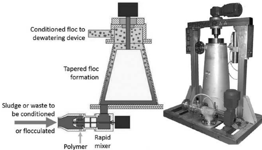
Figure B.5 In-line rapid mixing and tapered flocculation device for sludge conditioning (courtesy Aqueen Aqua-Engineering GmbH, www.aqueen.de ).
