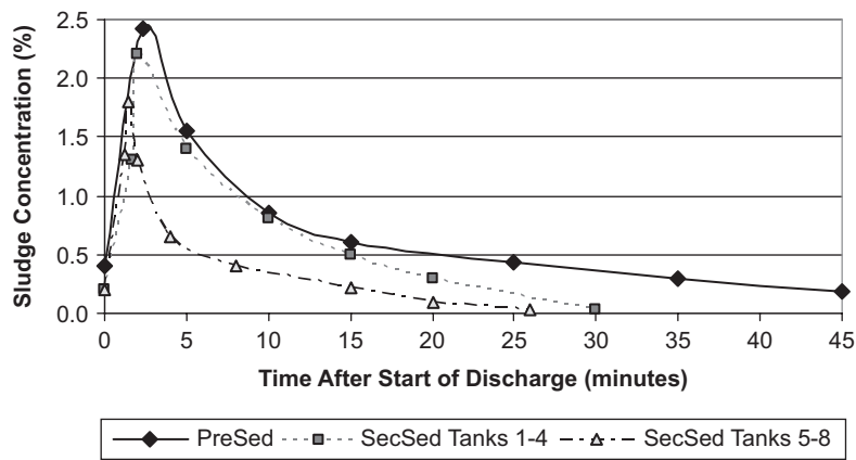
Figure B.15 Sedimentation tank sludge discharge concentrations with time (Bratby et al. 1993, 1996).
