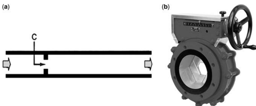
Figure 6.8 (a) Orifice plate within a pipe schematic. (b) Adjustable variable orifice diaphragm control valve (courtesy Emile Egger & Cia SA, www.eggerpumps.ch ).
