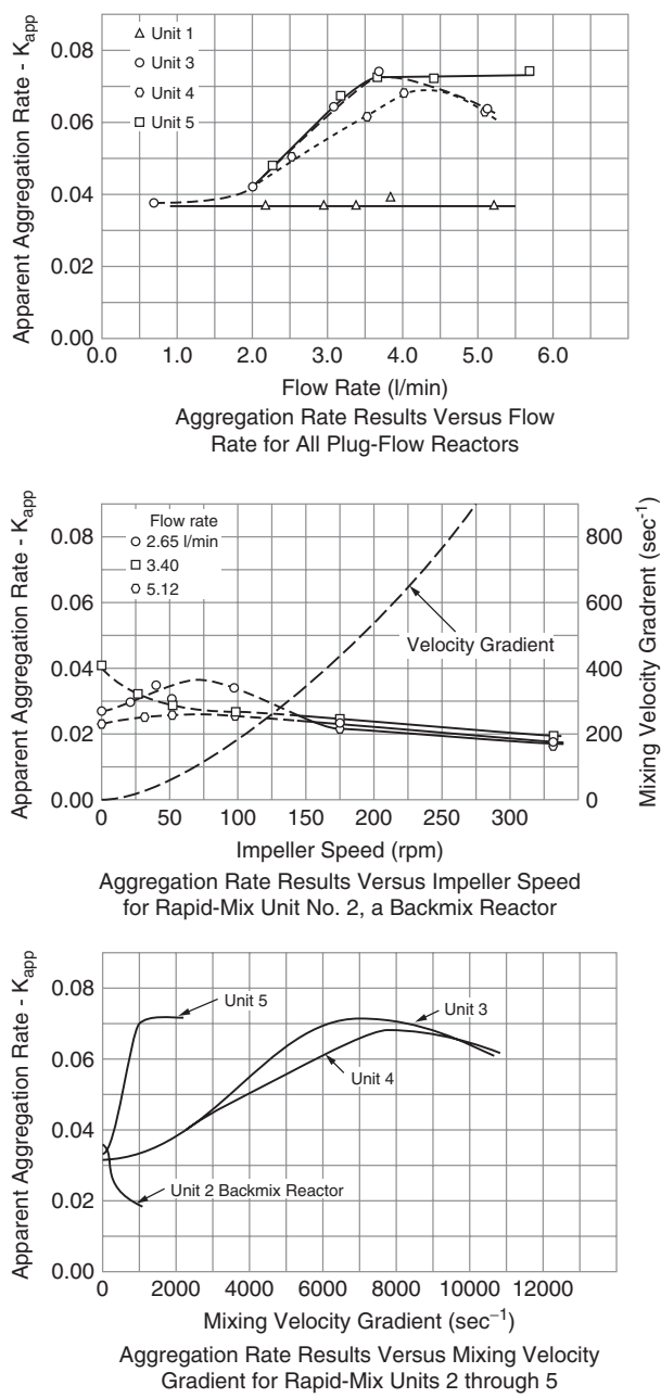
Figure 6.3 Results obtained using rapid mixers shown in Figure 6.2 (from Vrale & Jorden, 1971).
