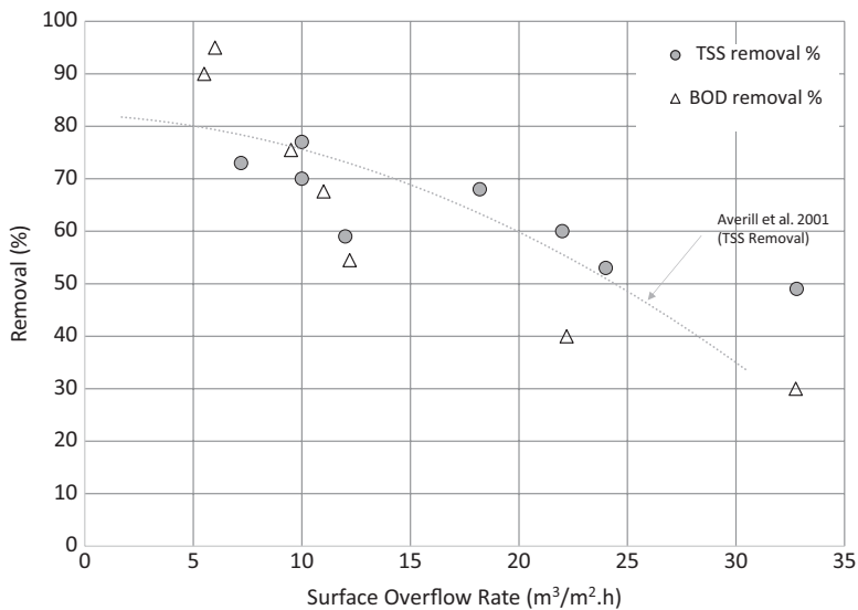
Figure 5.8 Effect of surface overflow rate (SOR) on TSS and BOD removals. (Adapted from Li et al. 2009. 1 m³/m² · h = 589 gpd/ft²).
