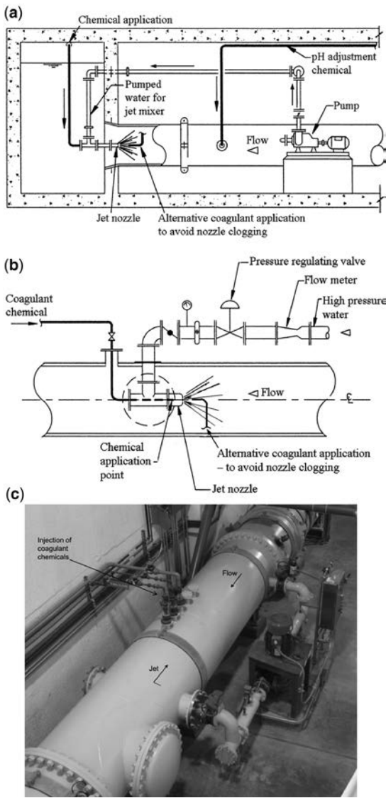
Figure 6.13 (a) In-line jet mixer with pumped injected flow (after Monk & Trussell 1991). (b) In-line jet mixer with plant pressurized flow (after Monk & Trussell 1991). (c) Example installation of an in-line jet mixer.
