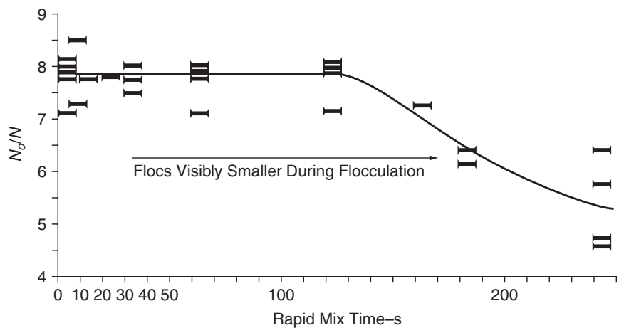
Figure 8.16 Optimizing rapid mix time. (Bratby, 1981).
