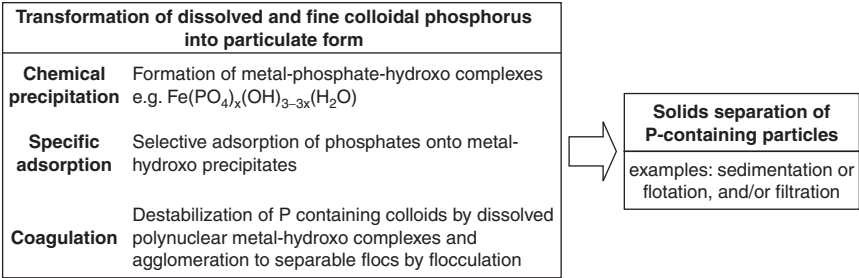
Figure 4.26 Overview of chemical precipitation and removal processes (after Maurer & Boller, 1999).
