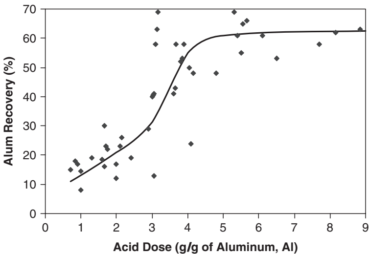
Figure B.29 Sulfuric acid dosage and alum recovery.
