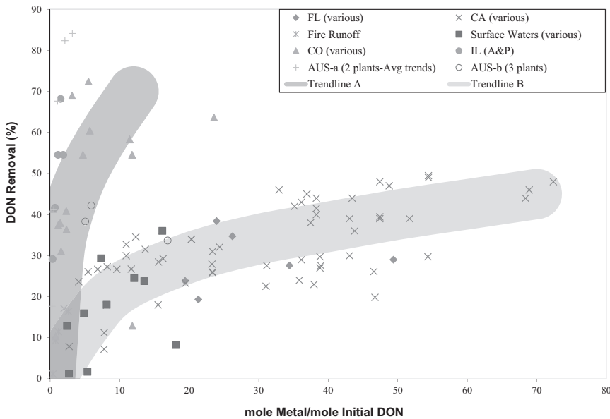
Figure 4.41 Compilation of Coagulant Dosages Required to Achieve DON Removals. The spread of results appears to follow two general trends.
