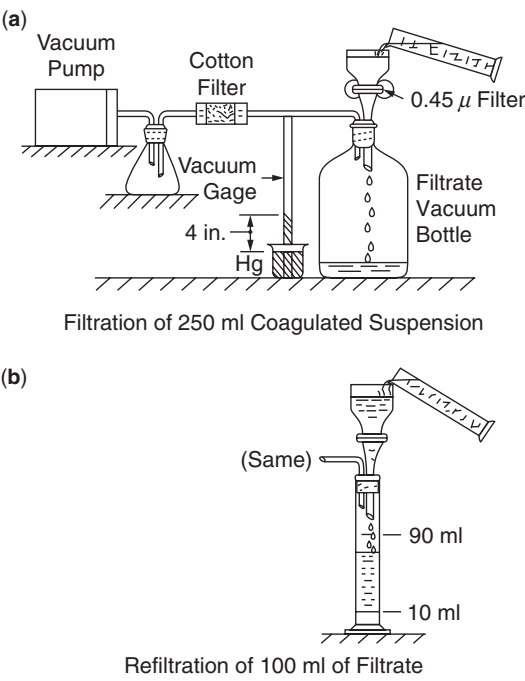
Figure 8.2 Apparatus for refiltration experiments. (From TeKippe & Ham, 1970).
