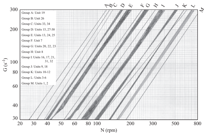
Figure 7.12 G values versus impeller speed, for the flocculation devices shown in Figures 7.11a through c.
