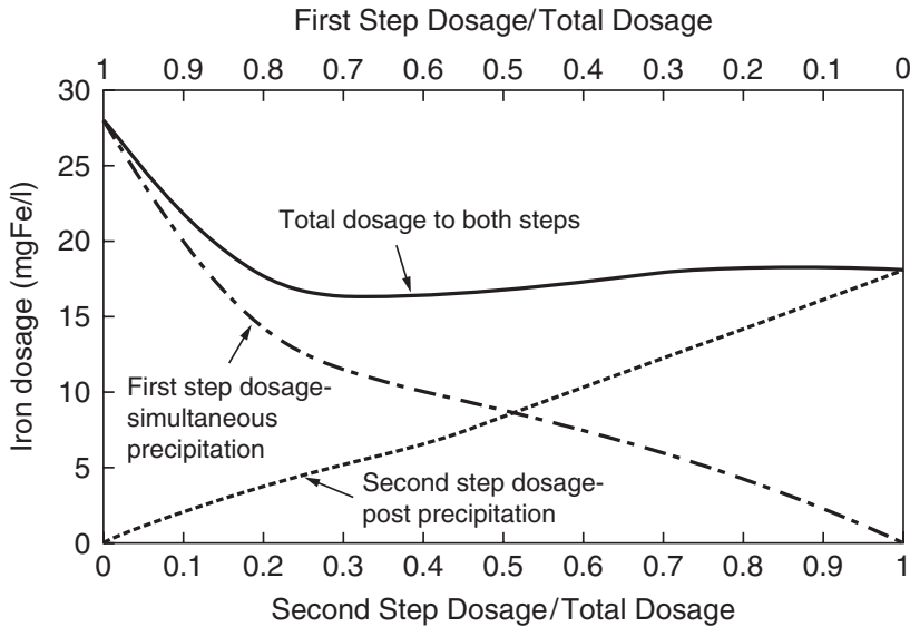
Figure 4.34 Relative dosages to first step simultaneous precipitation and second step direct filtration to achieve 0.1 mgP/l (after Maurer & Boller, 1999).
