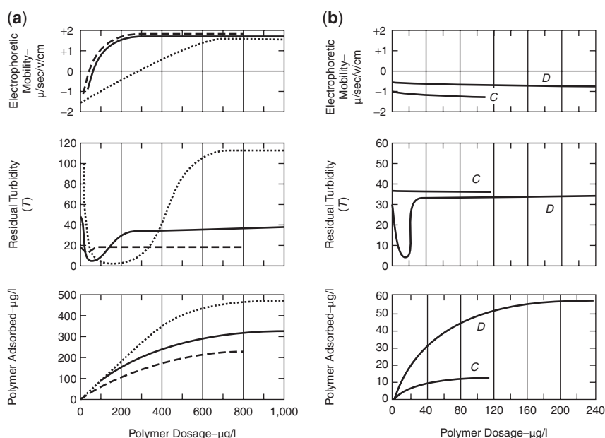
Figure 8.20 (a) Effect of initial clay concentration on destabilization of kaolin clay suspensions with cationic polymer: the dashed, solid and dotted curves represent clay concentrations of 14.9 mg/l, 29.8 mg/l and 73.2 mg/l respectively. (b) Effect of \text{CaCl}_2 on destabilization of kaolin clay suspensions with anionic polymer: the kaolin suspensions (33.3 mg/l) contain 25 mg/l \text{CaCl}_2 (curve C) and 250 mg/l \text{CaCl}_2 (curve D). (From Black et al. 1965.)
