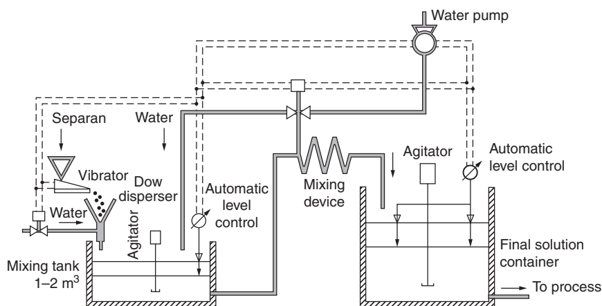
Figure 3.9 Continuous type polymer dissolution system (courtesy Dow Chemicals).
