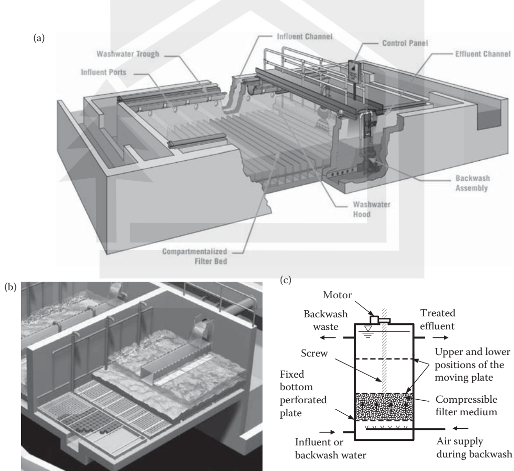
FIGURE 15.9 Proprietary filter systems: (a) traveling-bridge filter (Courtesy SUEZ), (b) pulsed-bed filter (Courtesy Evoqua Water Technologies), and (c) synthetic medium filter (or Fuzzy filter).
