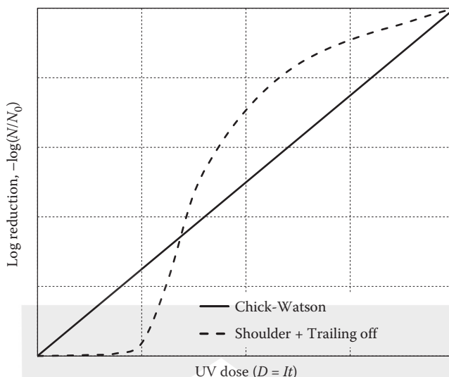
FIGURE 11.23 Typical deviations from Chick-Watson model observed in UV irradiation disinfection.
