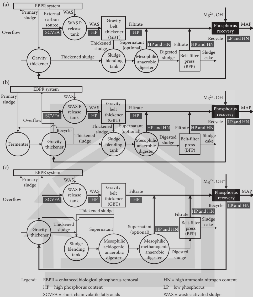
FIGURE 13.36 Conceptual process diagrams for phosphorus recovery using different carbon source alternatives: (a) Train 1: external carbon source, (b) Train 2: overflow from fermenter/thickener, and (c) Train 3: supernatant from acid phase reactor of A/GAnD process (Example 13.57).
