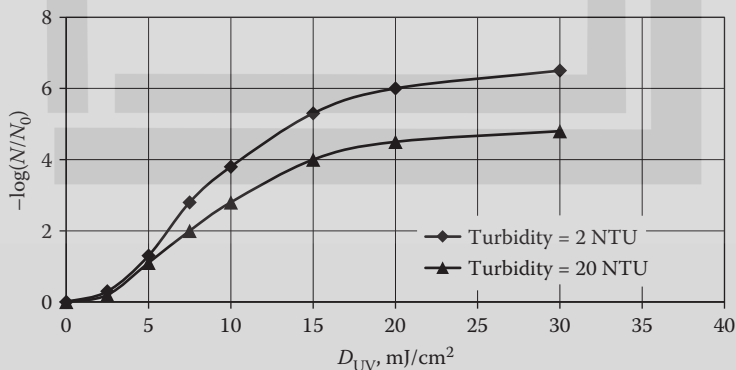
FIGURE 11.25 Plot of -\log(N/N_0) versus D_{UV} (Example 11.59).
