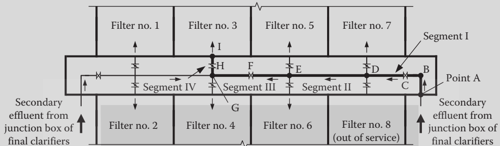
FIGURE 15.13 Filter influent piping details (Example 15.23).
