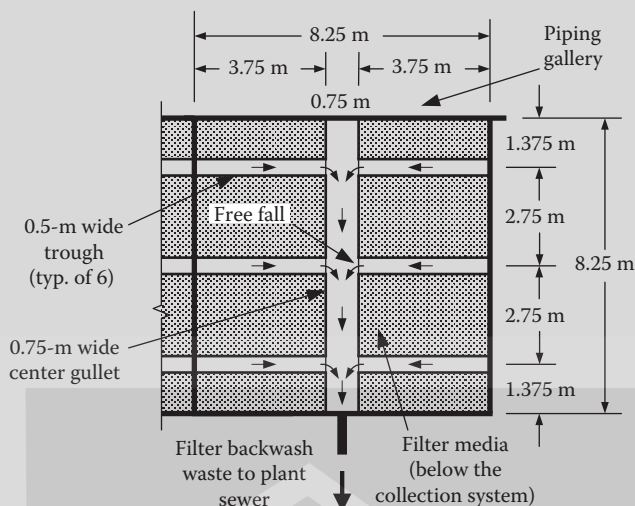
FIGURE 15.18 Conceptual layout of backwash waste collection system (Example 15.31).
