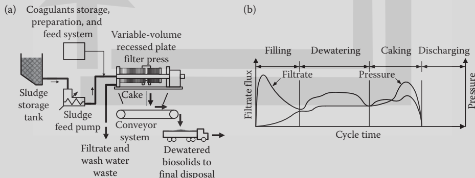
FIGURE 13.29 Design of variable-volume recessed plate filter press: (a) process flow diagram and (b) definition sketch of functional stages in operating cycle (Example 13.49).
