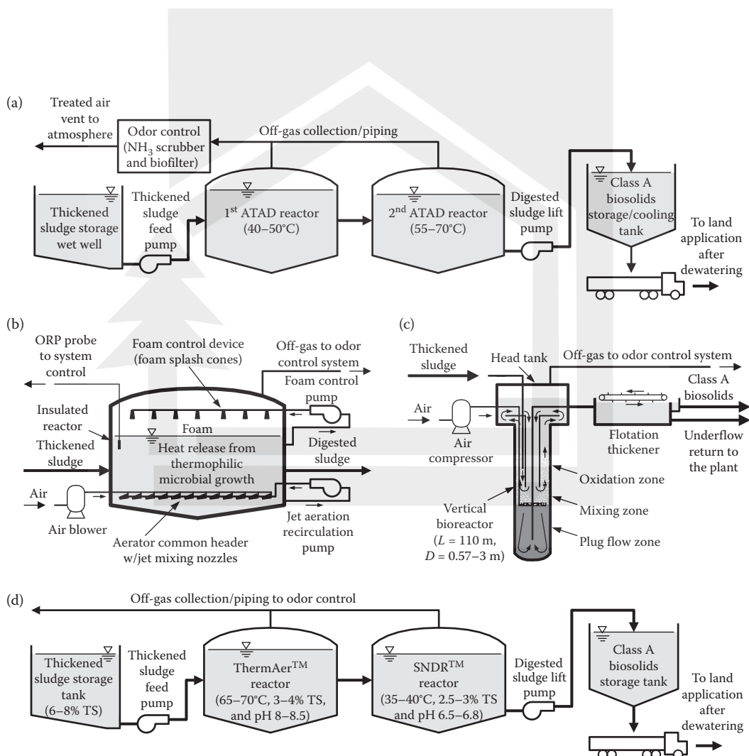
FIGURE 13.18 Autothermal thermophilic aerobic digestion (ATAD) processes: (a) schematic flow diagram of a two-stage ATAD system, (b) major components of the ATAD reactor, (c) VERTAD™ system, and (d) schematic flow diagram of ThermAer™/SNDR™ system.
