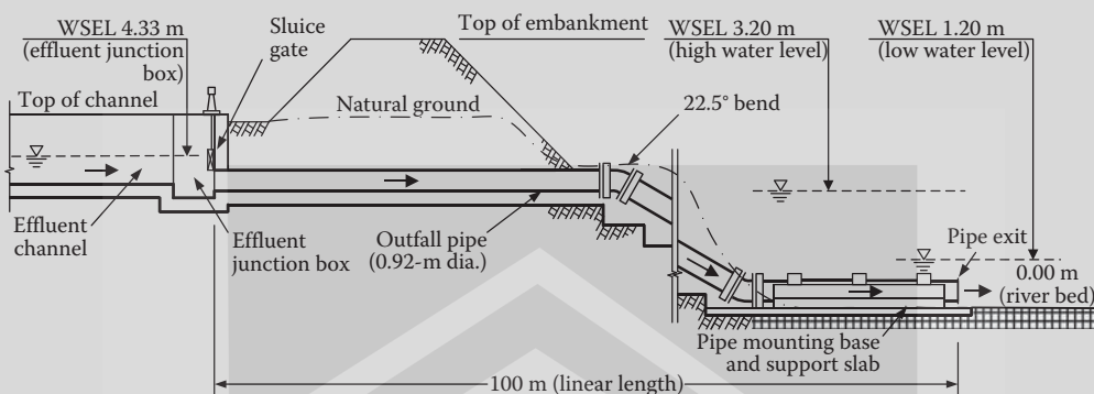
FIGURE 12.13 Conceptual side view of the outfall structure and hydraulic profile (Example 12.40).
