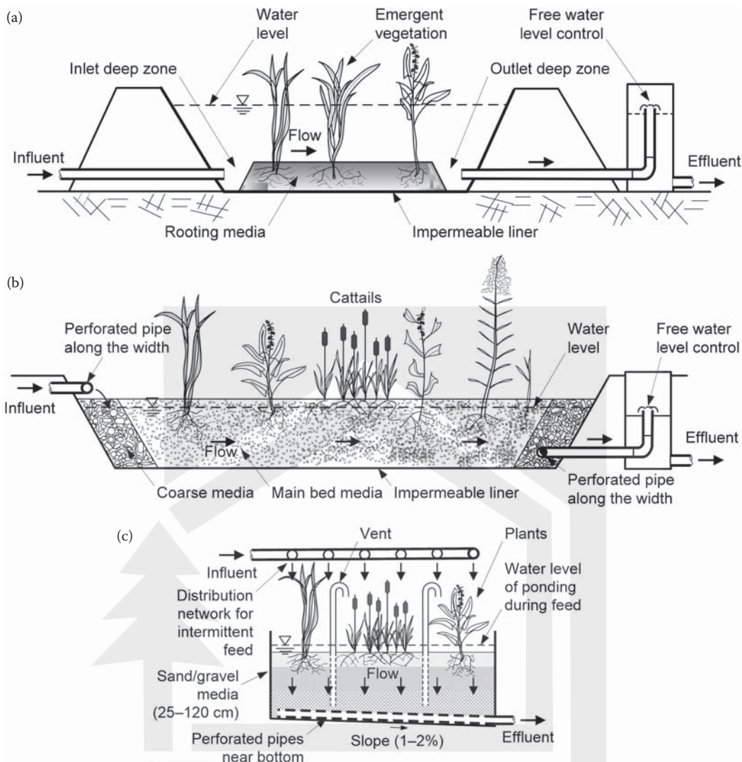
FIGURE 15.2 Constructed wetlands: (a) free water surface (FWS), (b) horizontal subsurface flow (HSF), and (c) vertical flow (VF). (Adapted in part from References 3, 10, 19, 21, and 22.)
